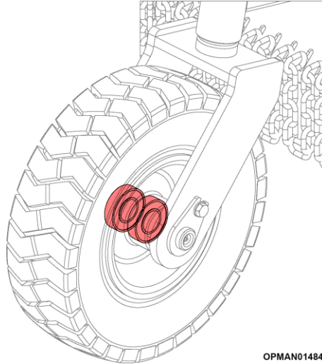
Figure 5.42 – Multicut Wheel Bearing
