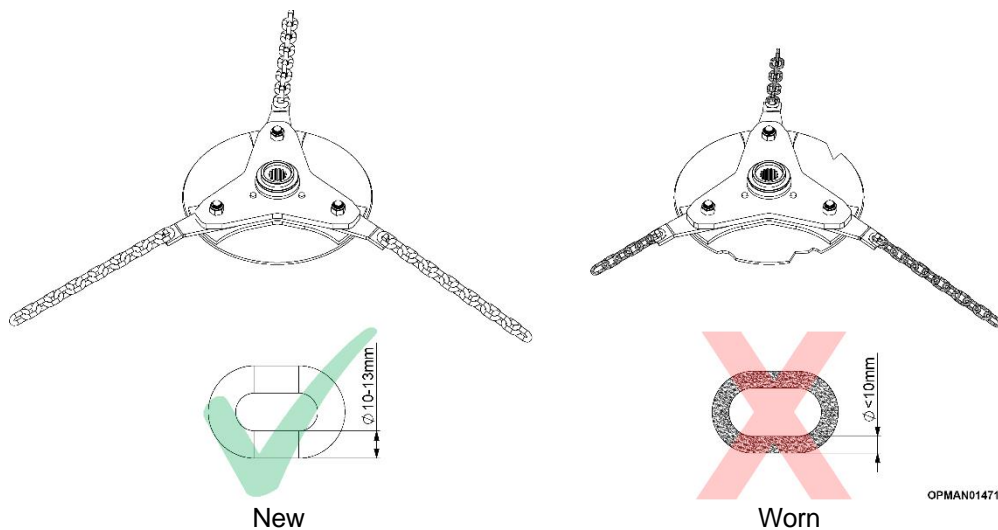
Figure 5.28 - Multicut Chains
