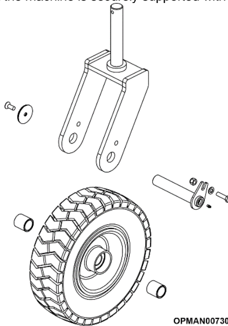
Figure 5.41 – Multicut Wheel & Fork Assembly
