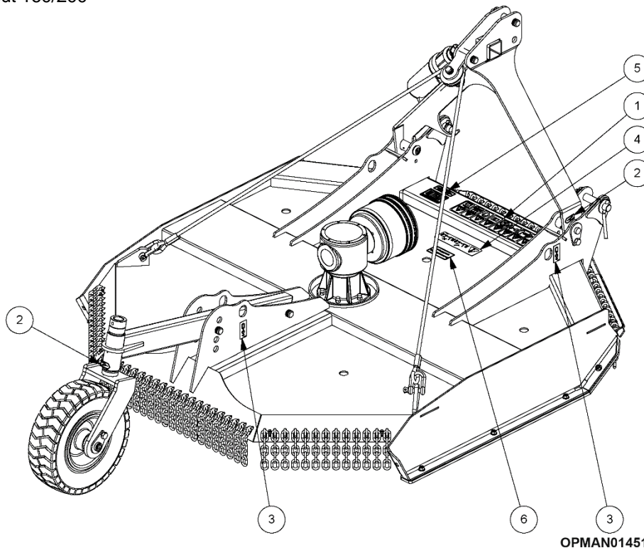
Figure 2.4 – Multicut 160/200 Safety & Instructional Decal Placement
