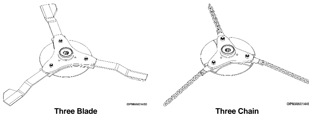
Figure 5.25 – Blade/Chain Carrier Options
