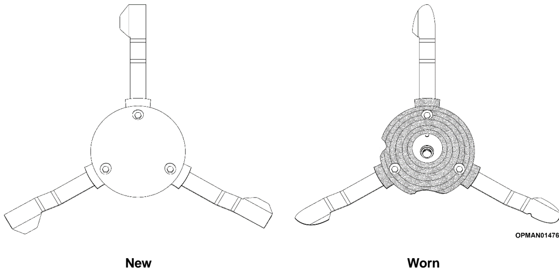
Figure 5.32 New vs Worn Anti-scalp Dish Comparison (Blade set-up shown)
