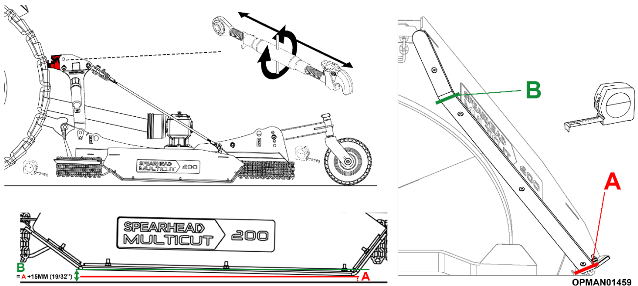
Figure 4.9 – Multicut 160/200 Front To Rear Machine Levelling
