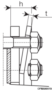
Figure 5.24 – Clutch Setting Dimension Guidance
