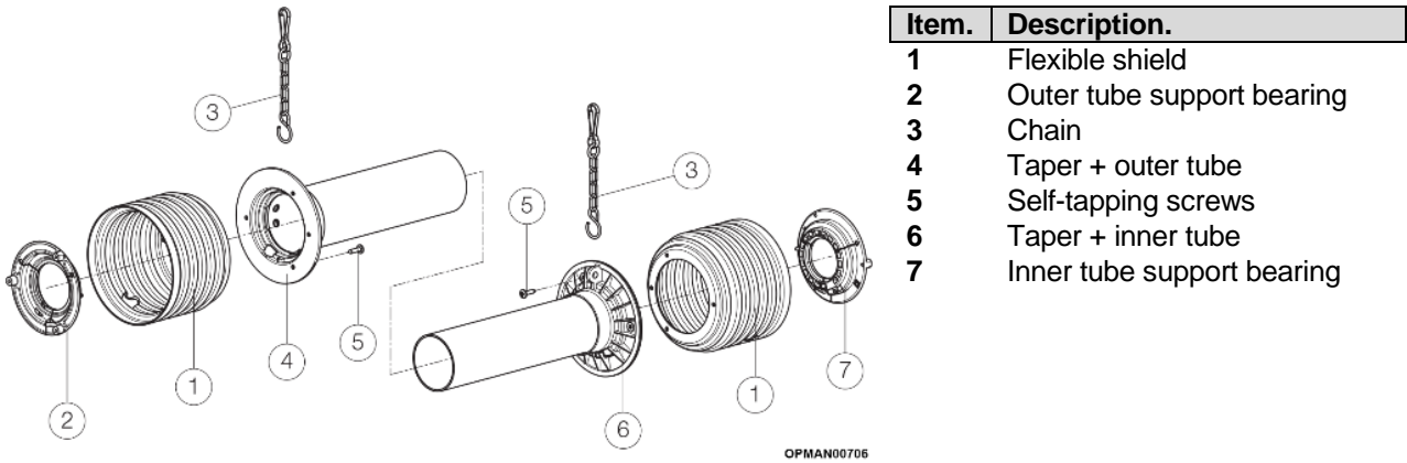
Figure 5.6/Table 5.6 - Input Shaft Safety & Wearing Components
