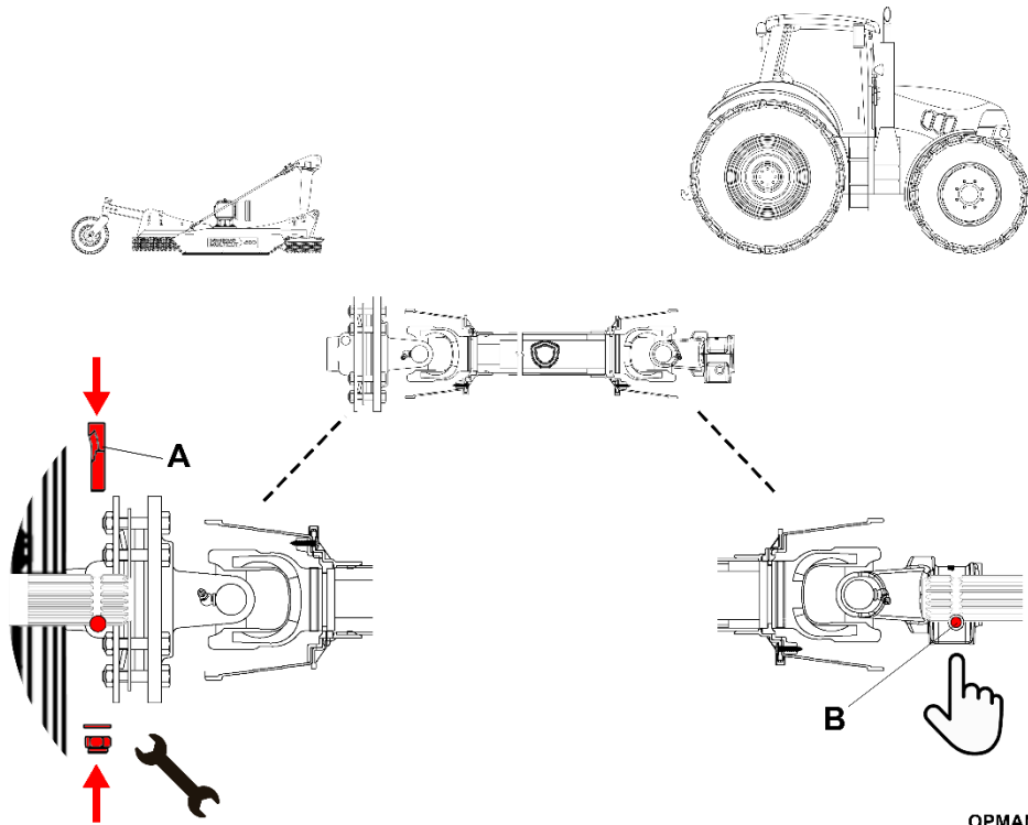
Figure 4.7 – Multicut Input Shaft Fitting & Removal
