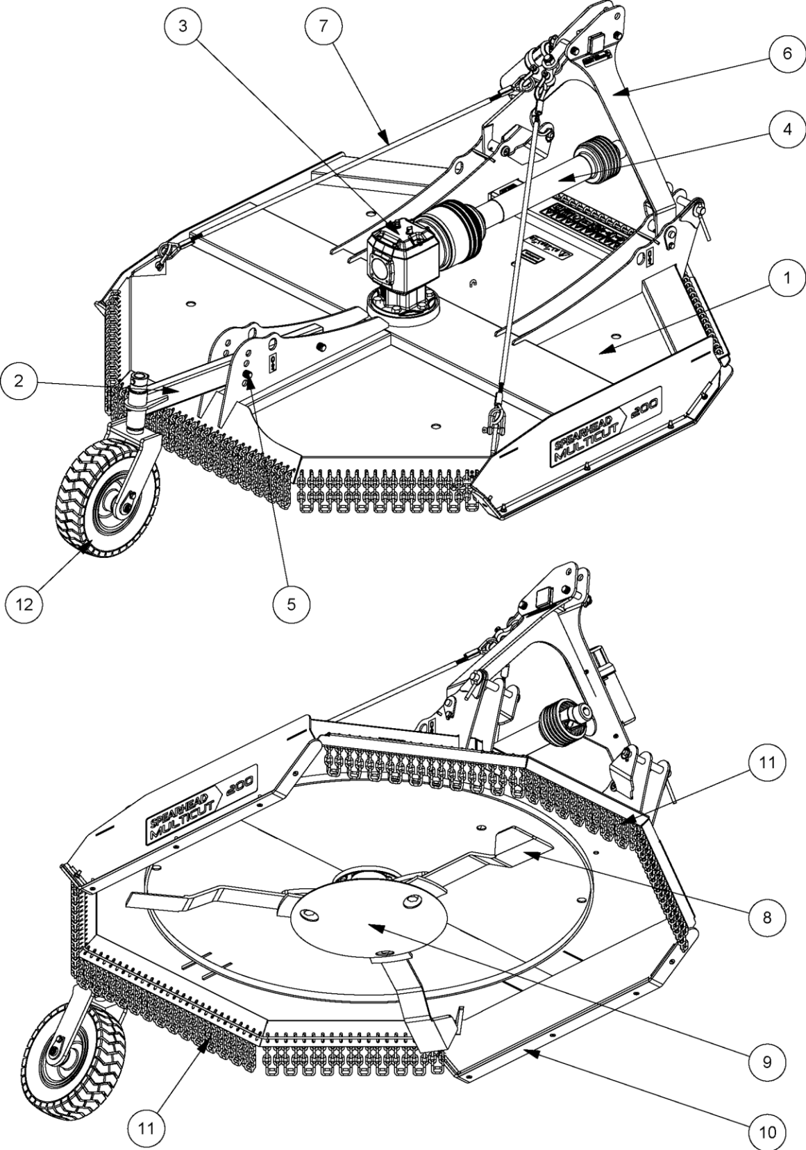
Figure 1.2 – Multicut 160/200 General Arrangement (200 model illustrated)
