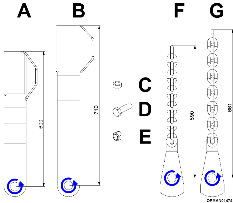
Figure 5.30 Multicut Range Blade & Chain Components
