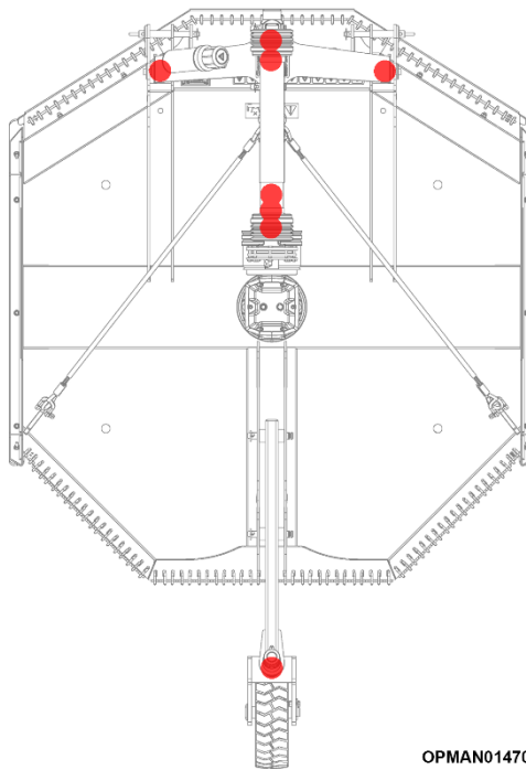
Figure 5.5 – Multicut Grease Point Locations
