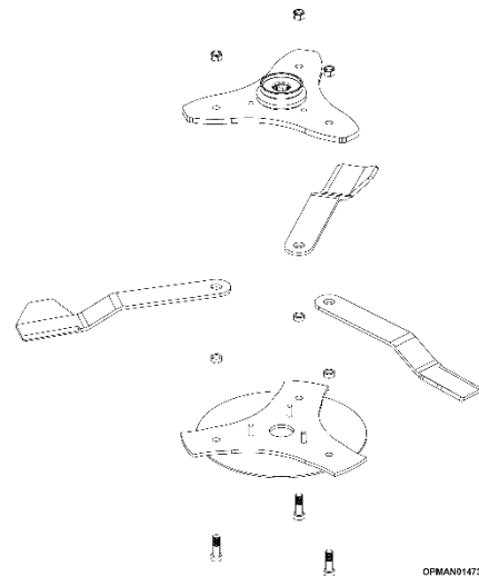
Figure 5.29 – Multicut Blade Carrier Assembly
