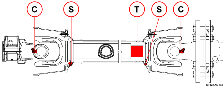
Figure 5.4 – Multicut Input Shaft Grease Locations
