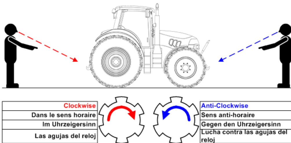
OPMAN00009 Figure 1.6 – Tractor PTO Shaft Rotation Definitions
