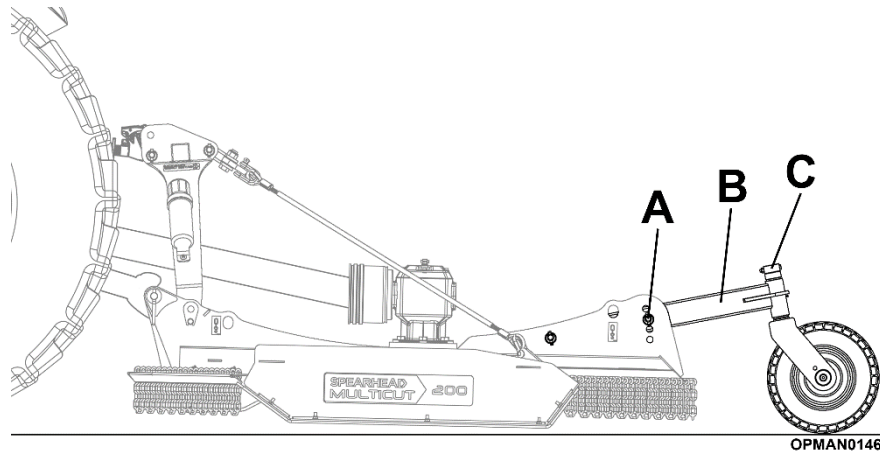
Figure 4.11 – Multicut 160/200 Height Adjustment Dependent Variables
