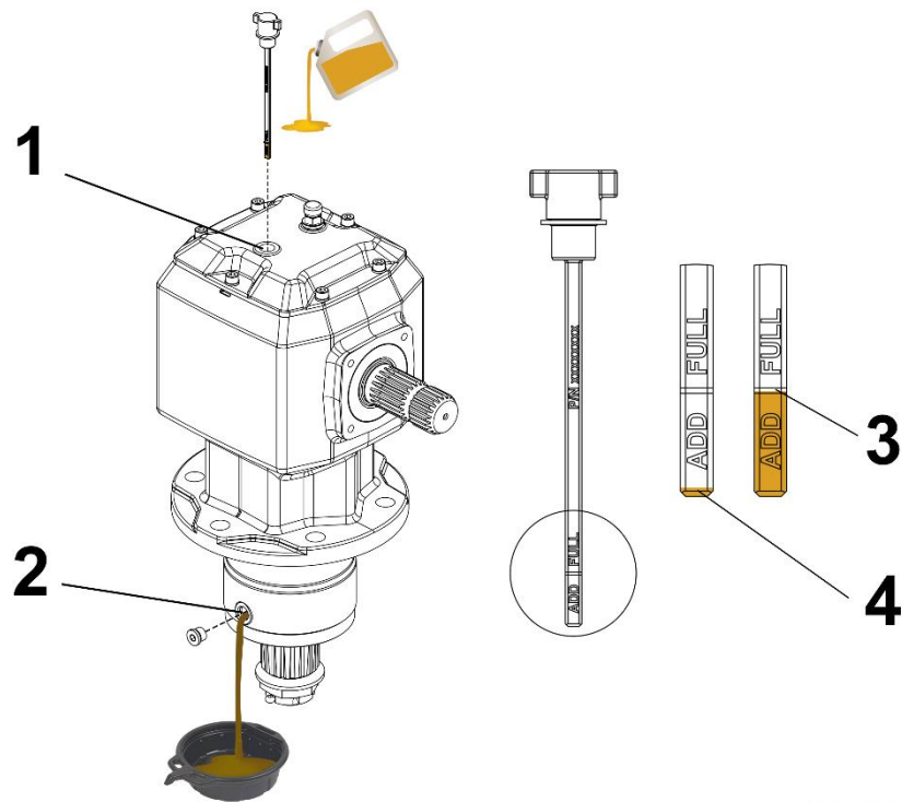
Figure 5.2 – Multicut Rotor Gearbox
