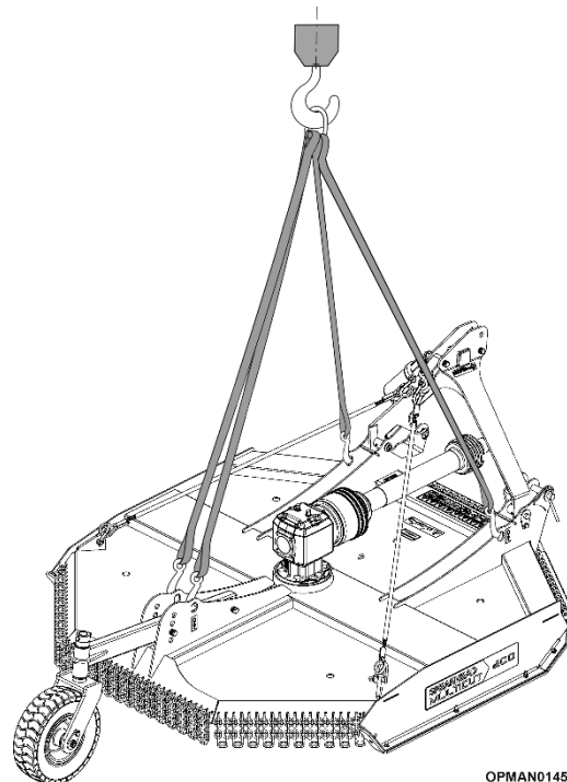
Figure 3.1 Shipping Position – Multicut 160/200
