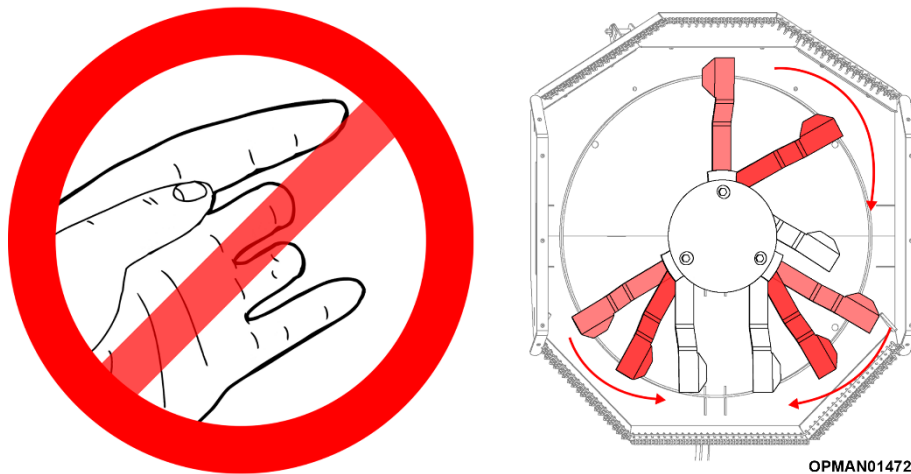
Figure 5.33 – Beware Of Falling Blades/Chains (Blades assembly shown)
