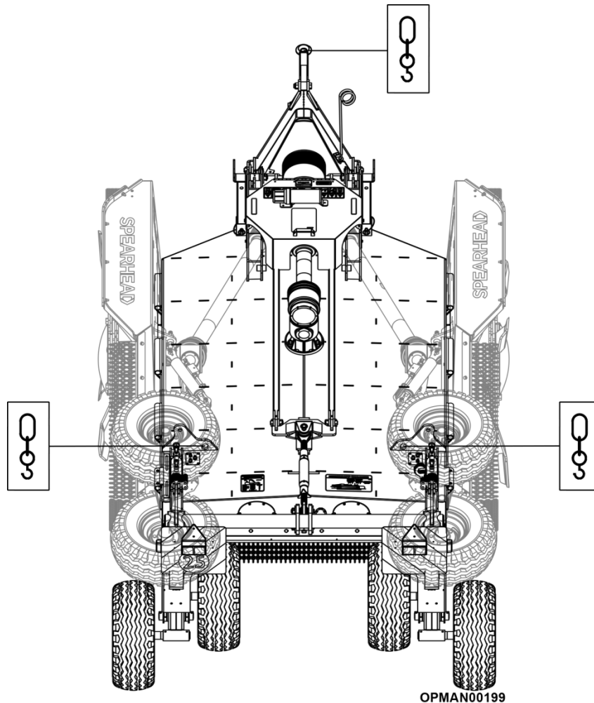
Figur 3.1 Forsendelsesposition – Stubble Master
