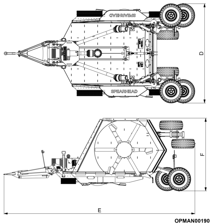
Figur 1.10 Transportdimensioner
